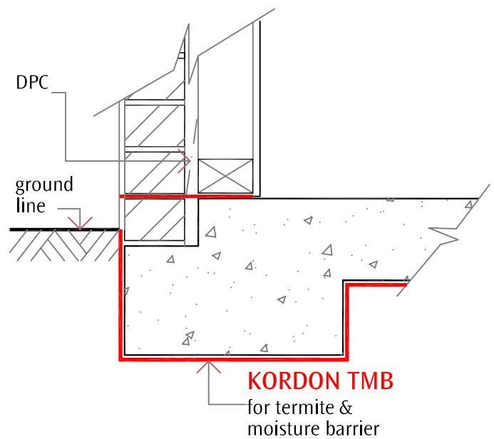
section detail 2
